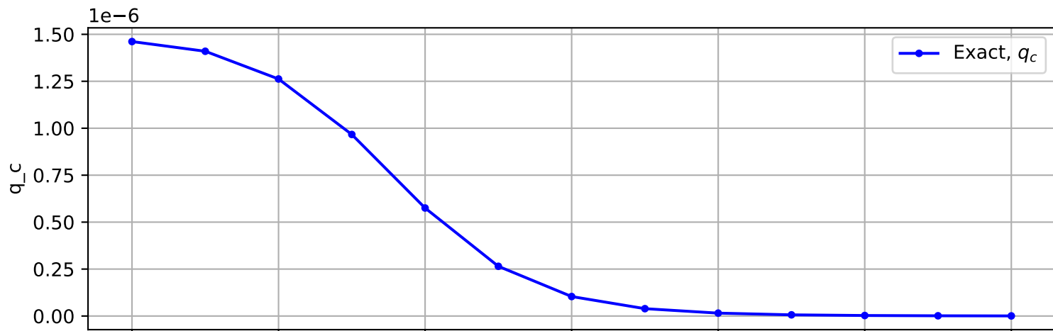
Trajectory No. 179
