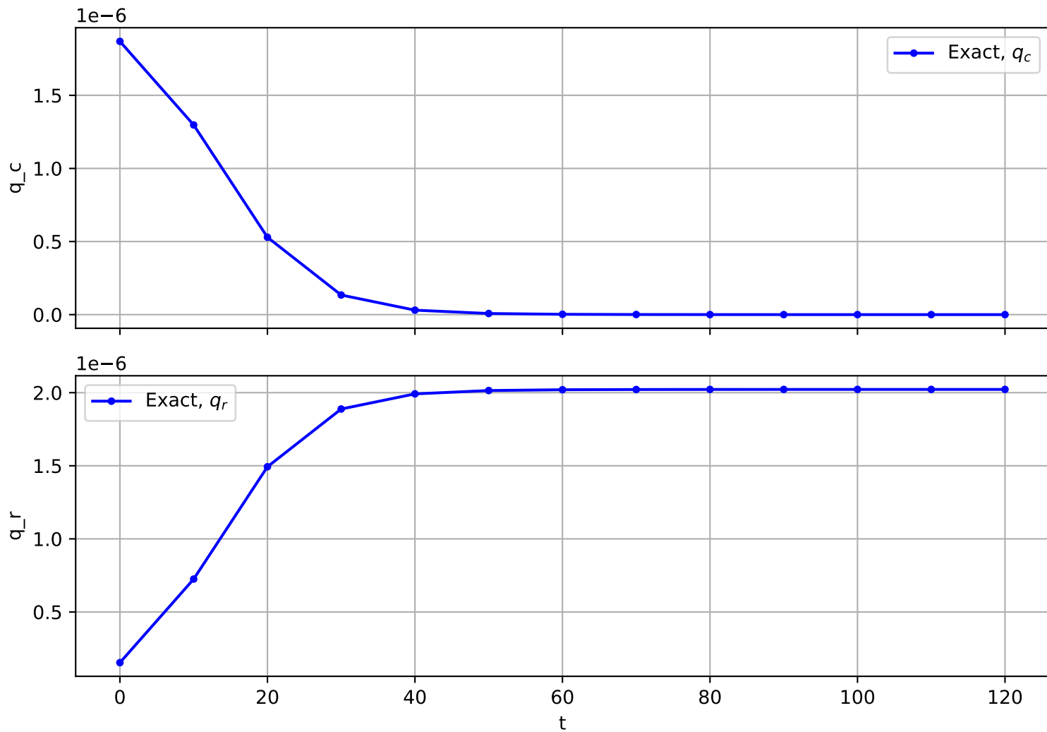
Trajectory No. 1797
