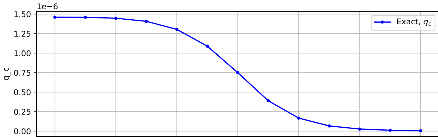
Trajectory No. 199
