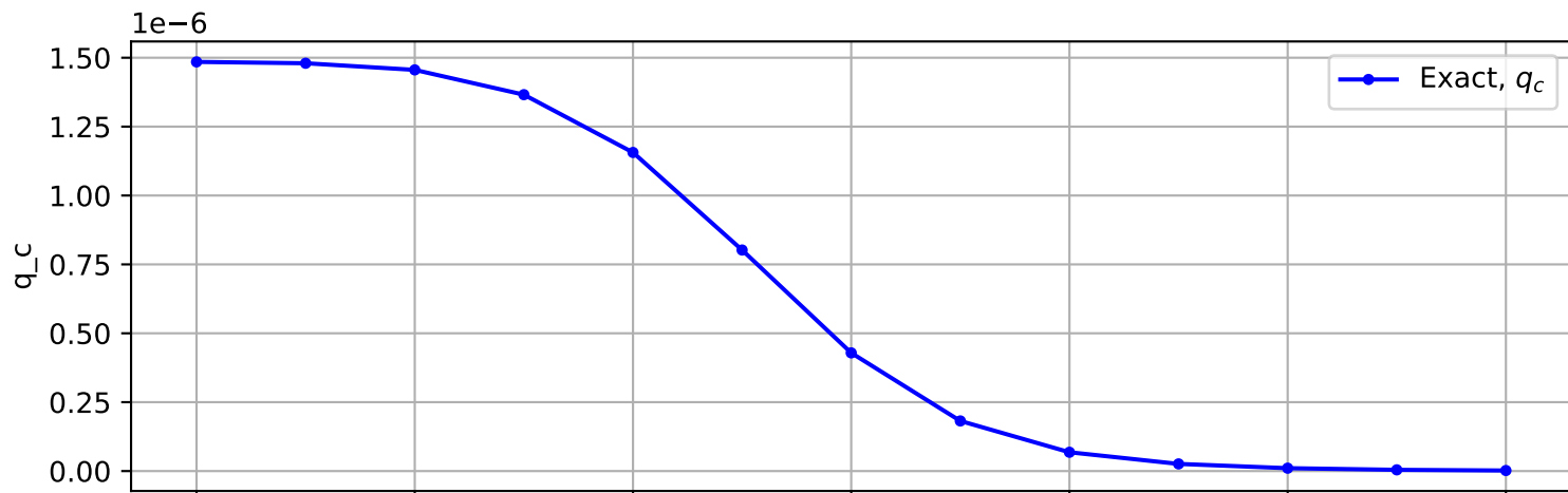
Trajectory No. 220
