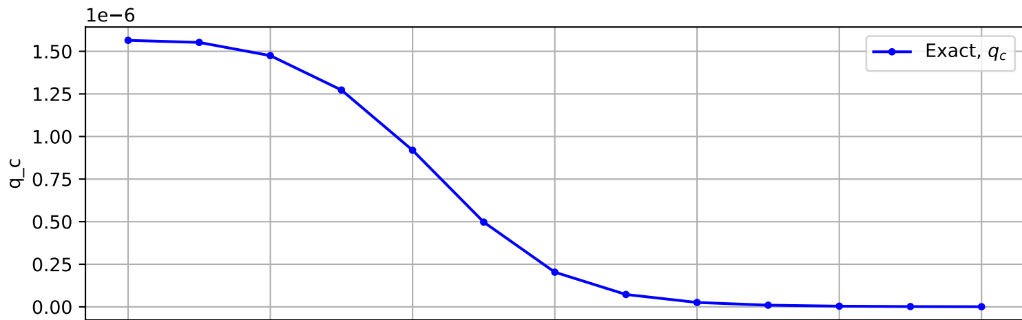
Trajectory No. 224
