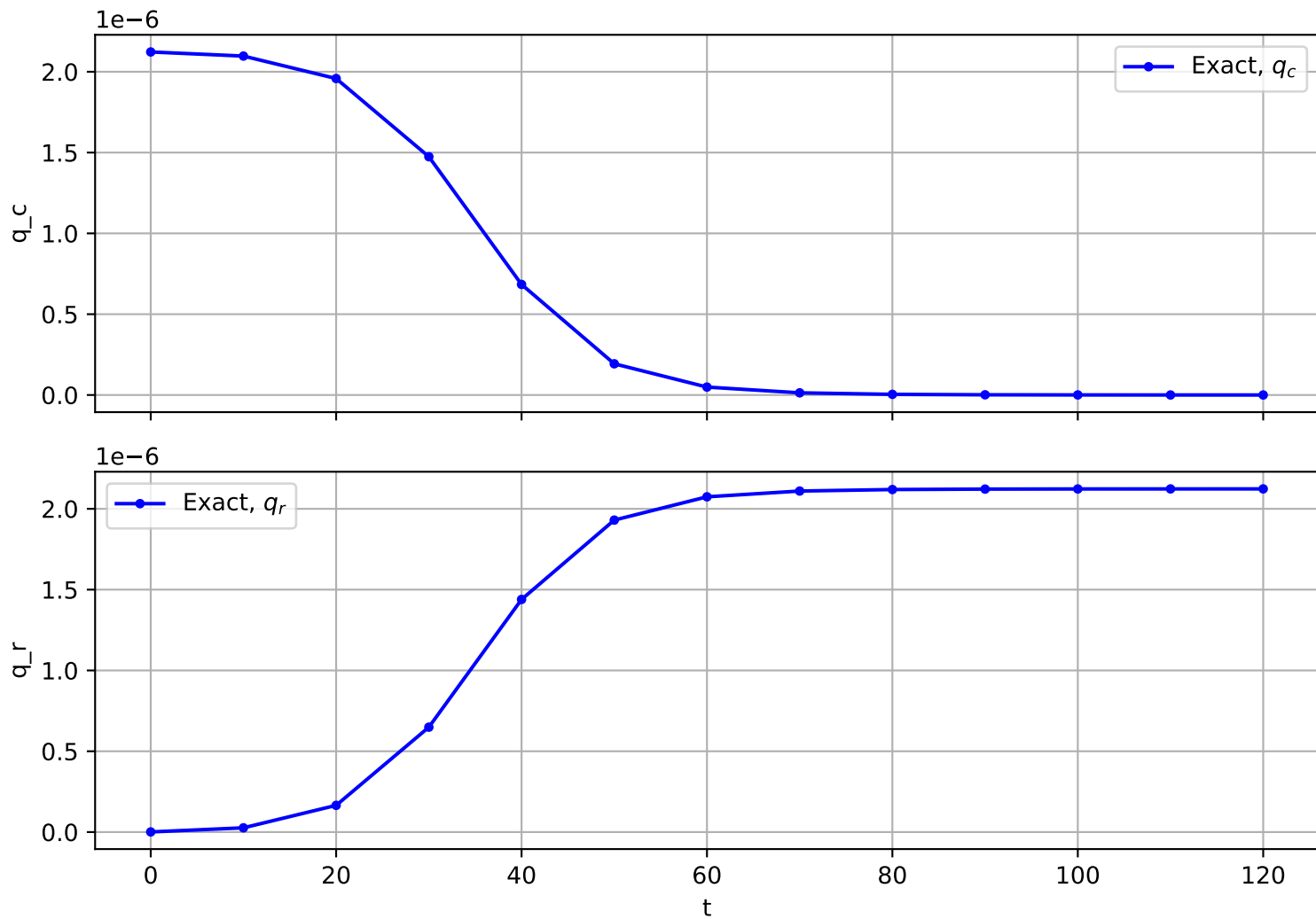
Trajectory No. 272
