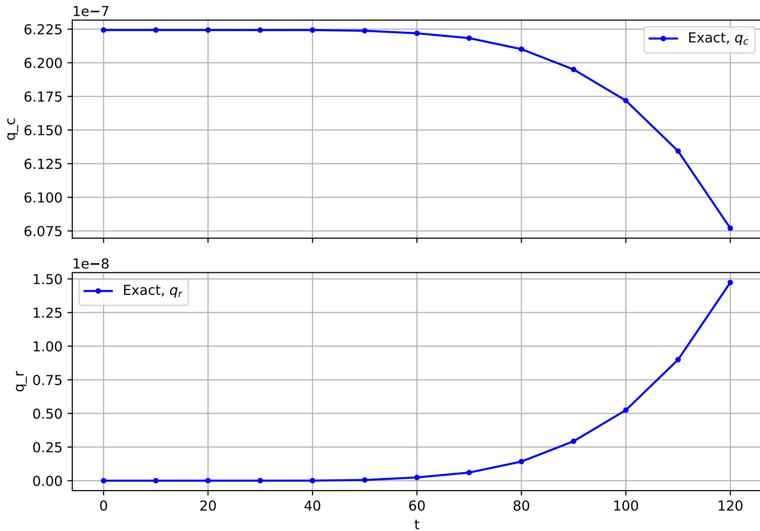
Trajectory No. 29
