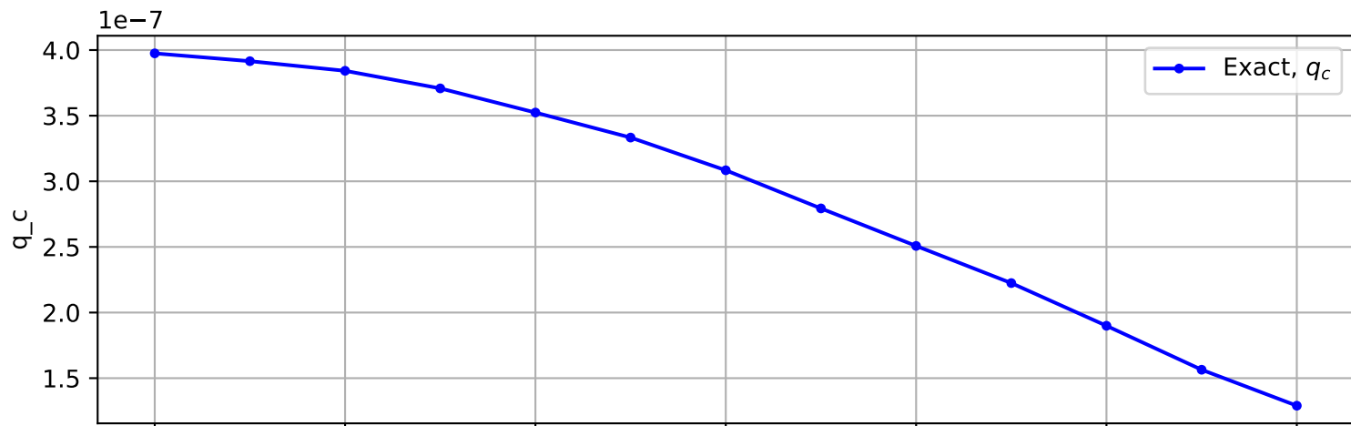
Trajectory No. 339
