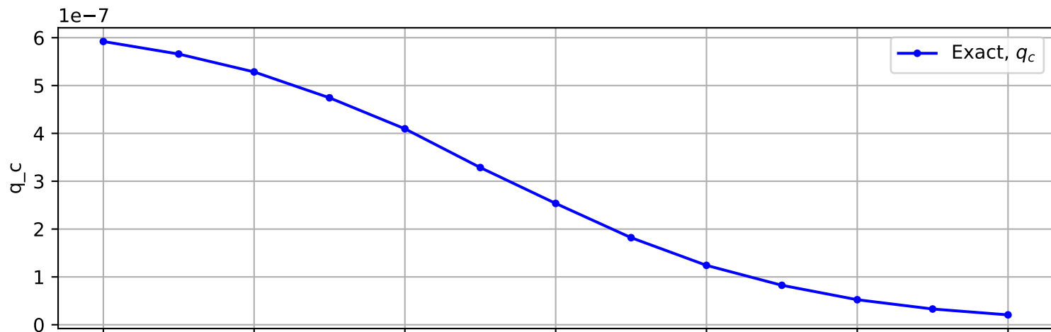
Trajectory No. 417
