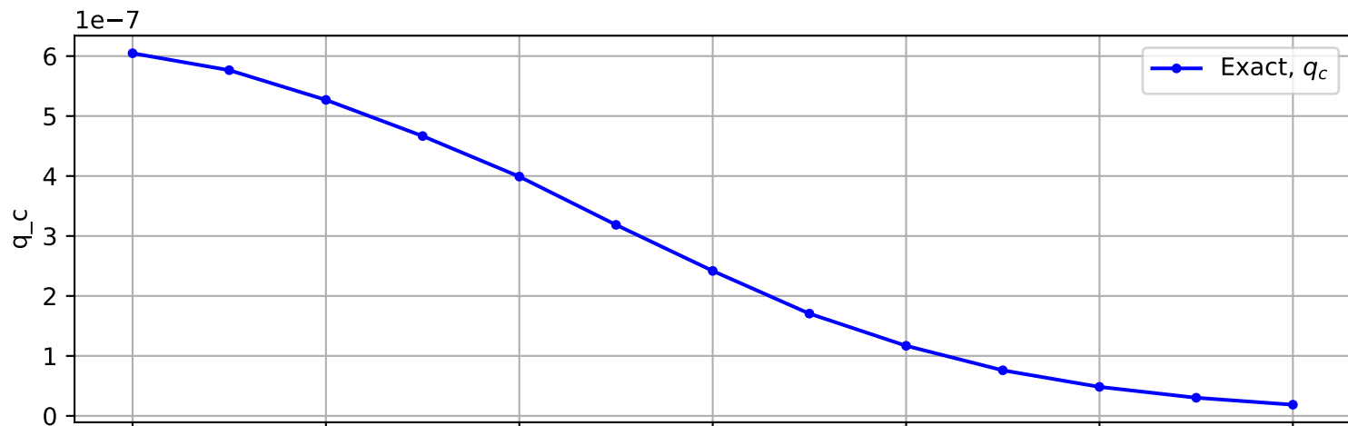
Trajectory No. 420
