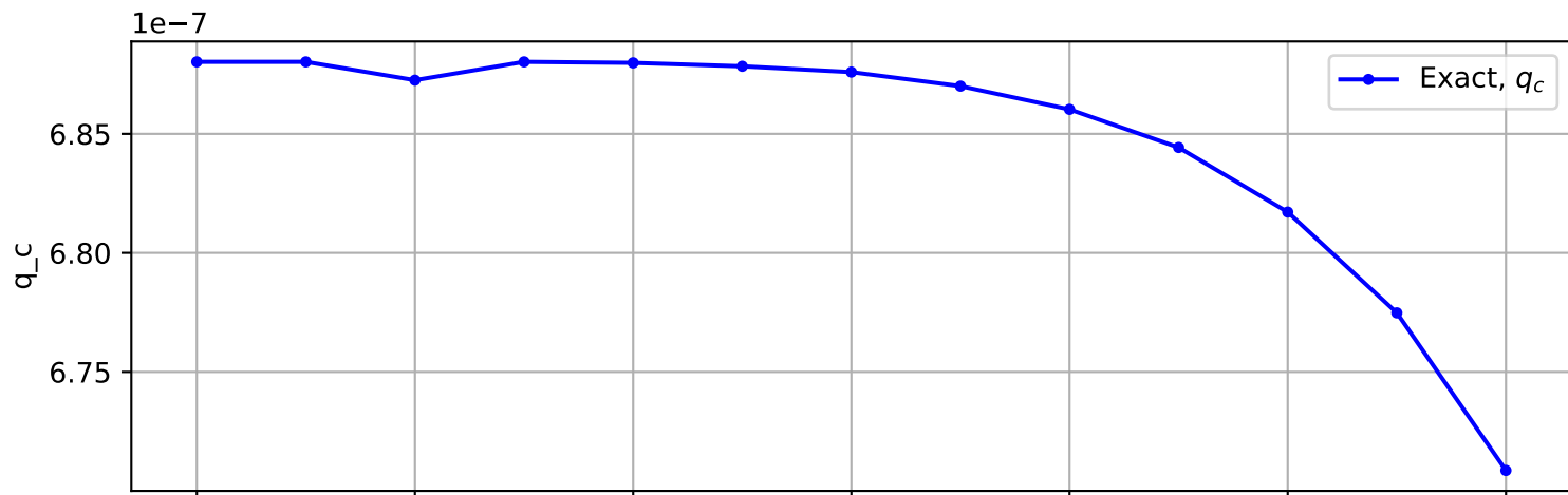
Trajectory No. 43
