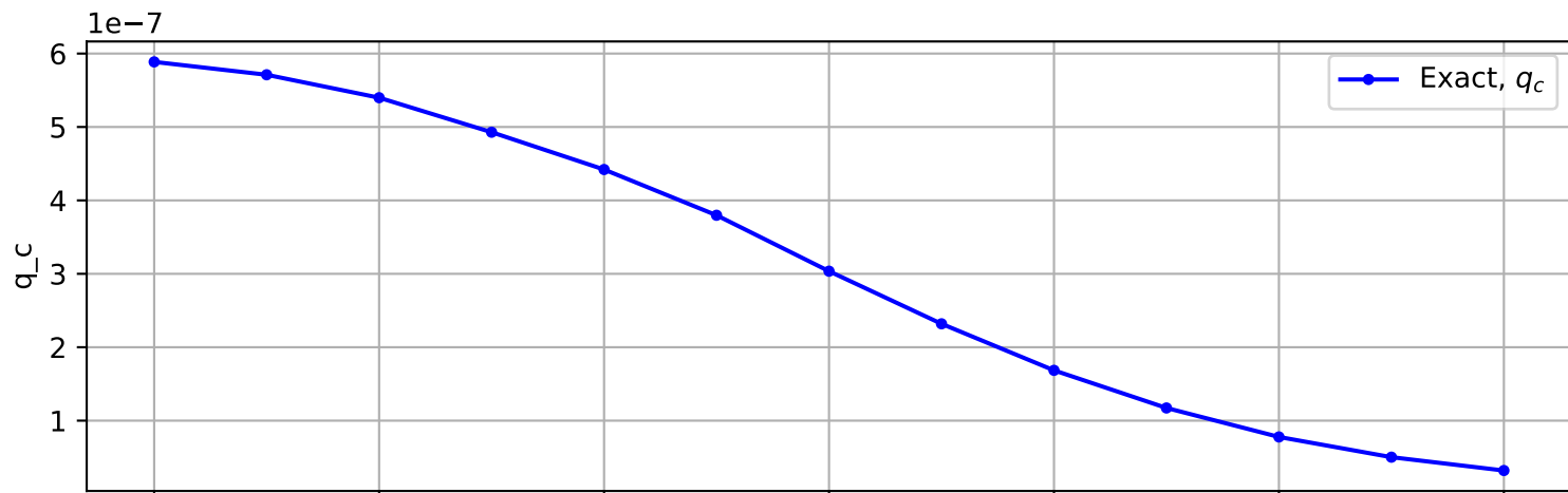
Trajectory No. 431
