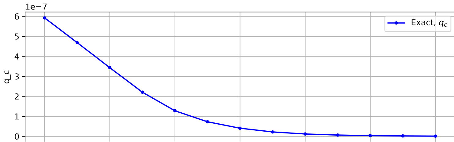
Trajectory No. 482
