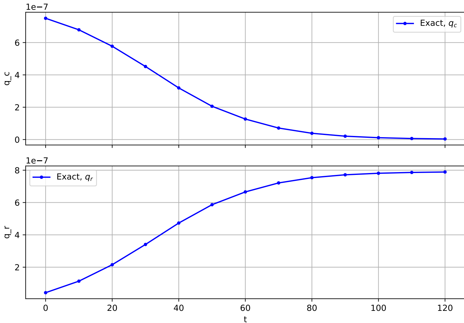
Trajectory No. 497
