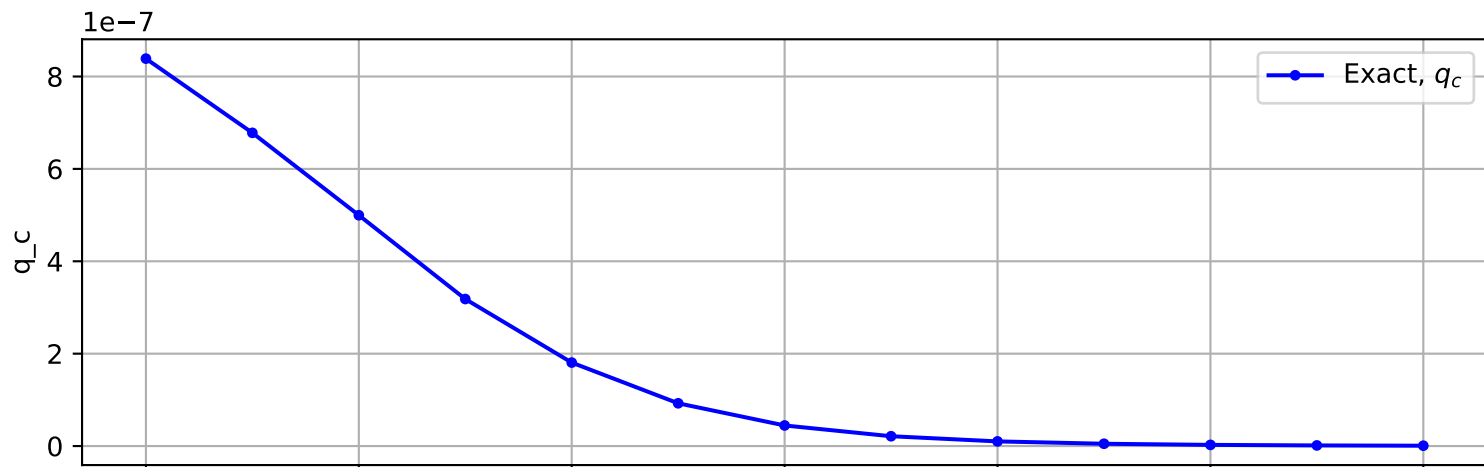
Trajectory No. 536
