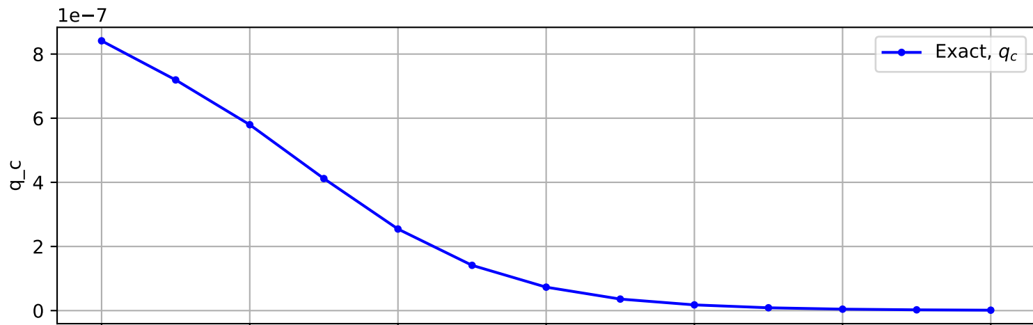
Trajectory No. 541
