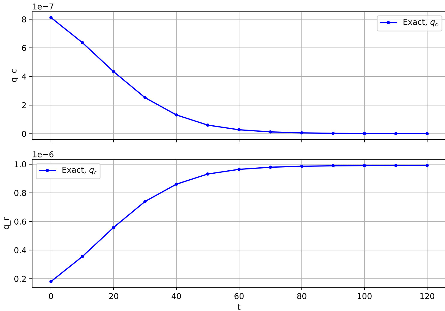
Trajectory No. 560
