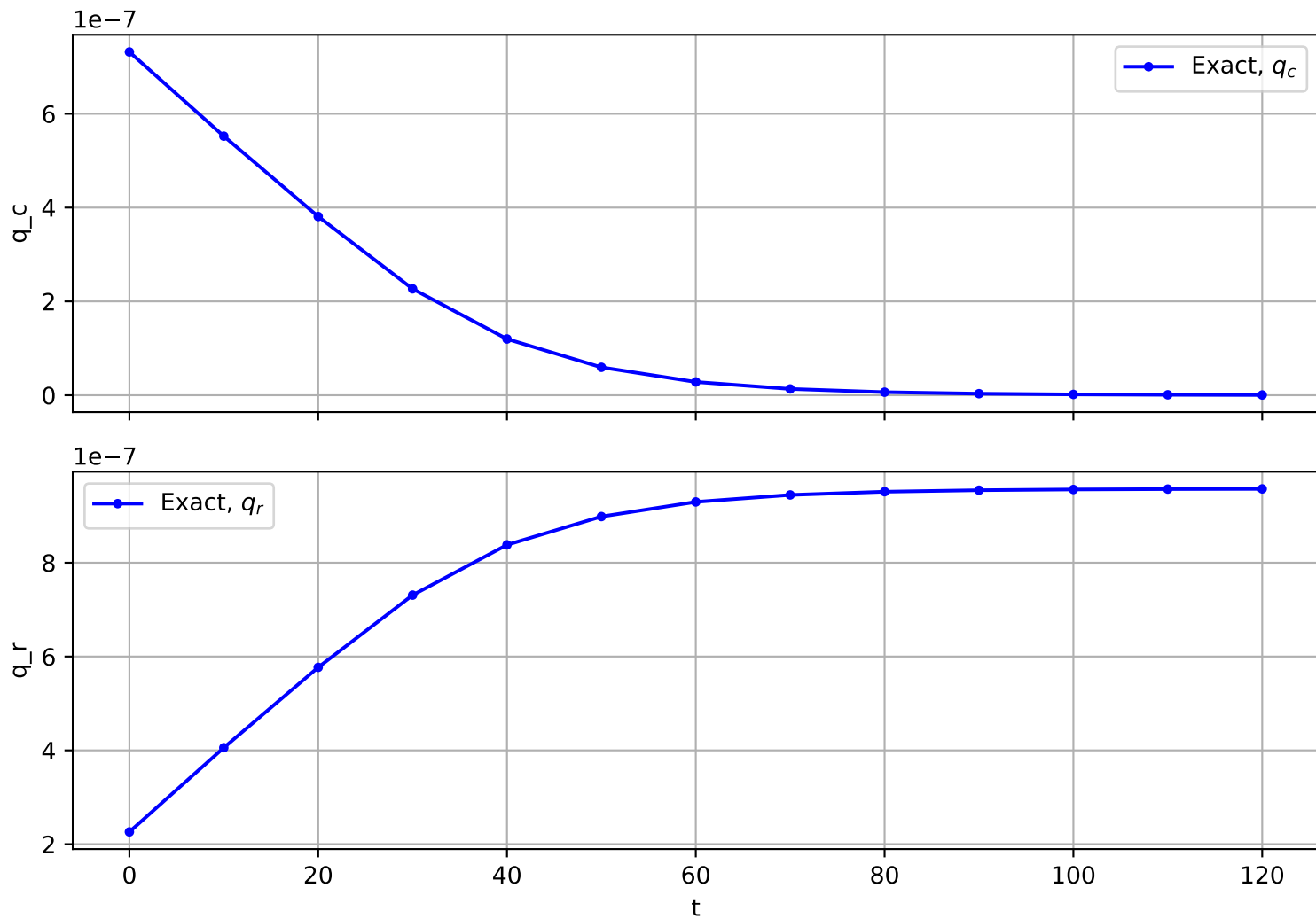
Trajectory No. 562
