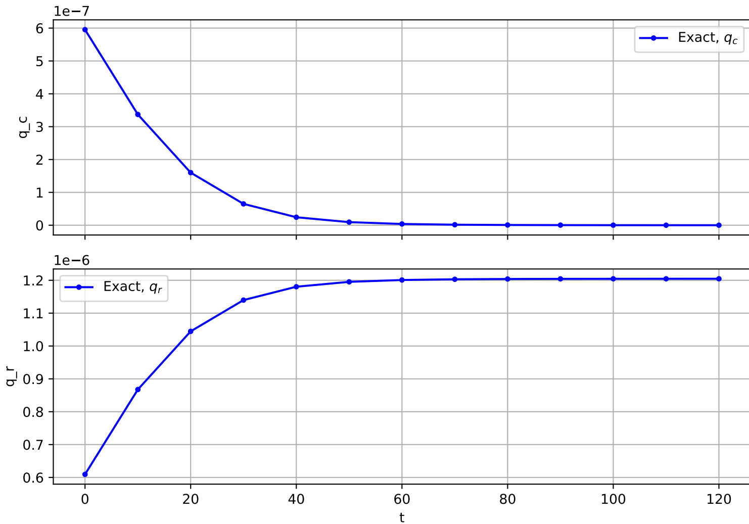
Trajectory No. 586
