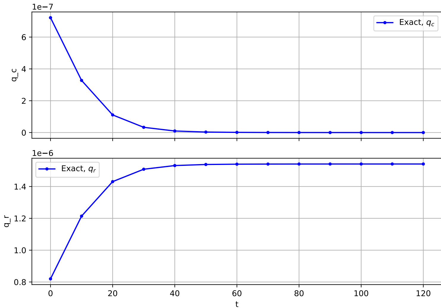
Trajectory No. 635
