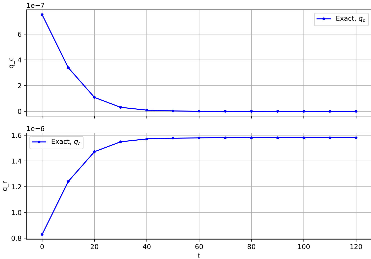
Trajectory No. 665
