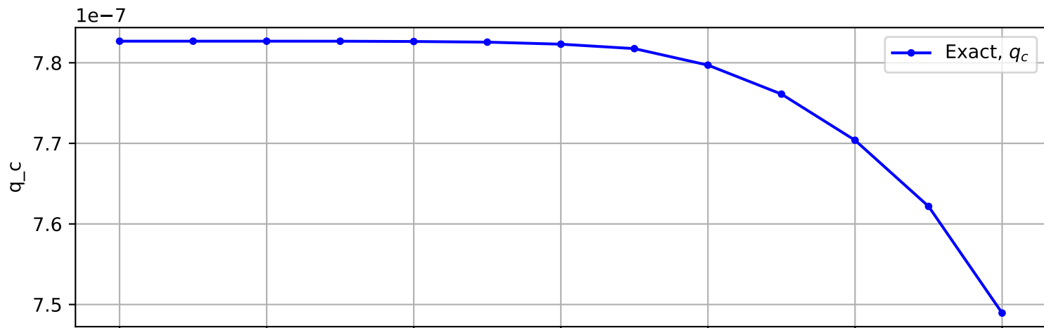
Trajectory No. 69
