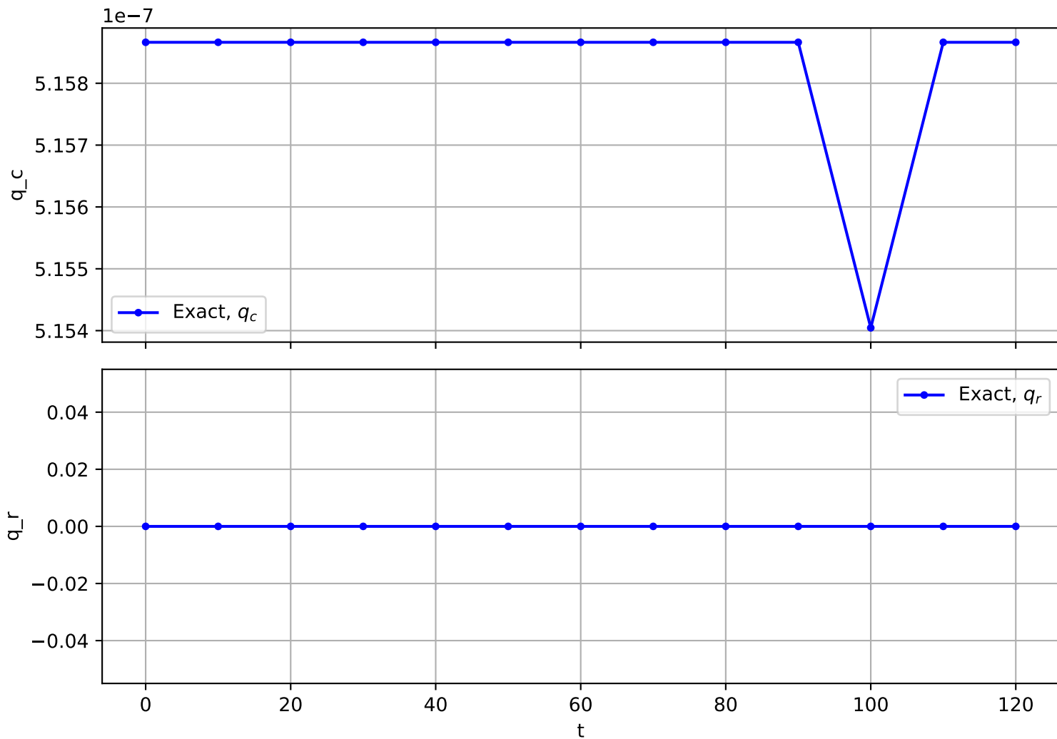
Trajectory No. 745
