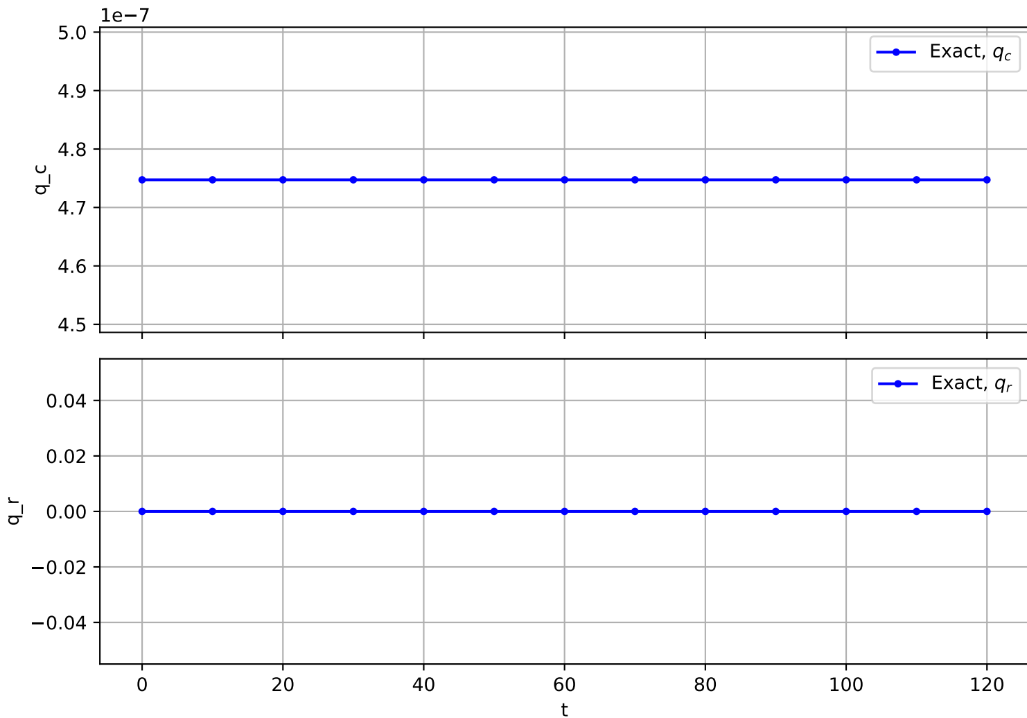
Trajectory No. 746
