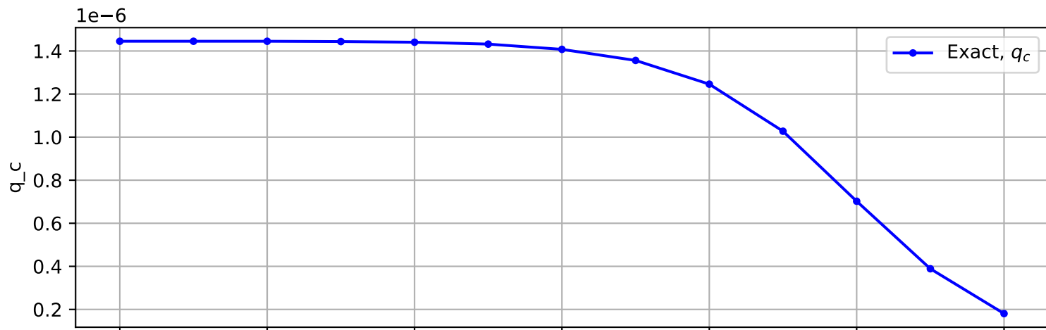
Trajectory No. 826
