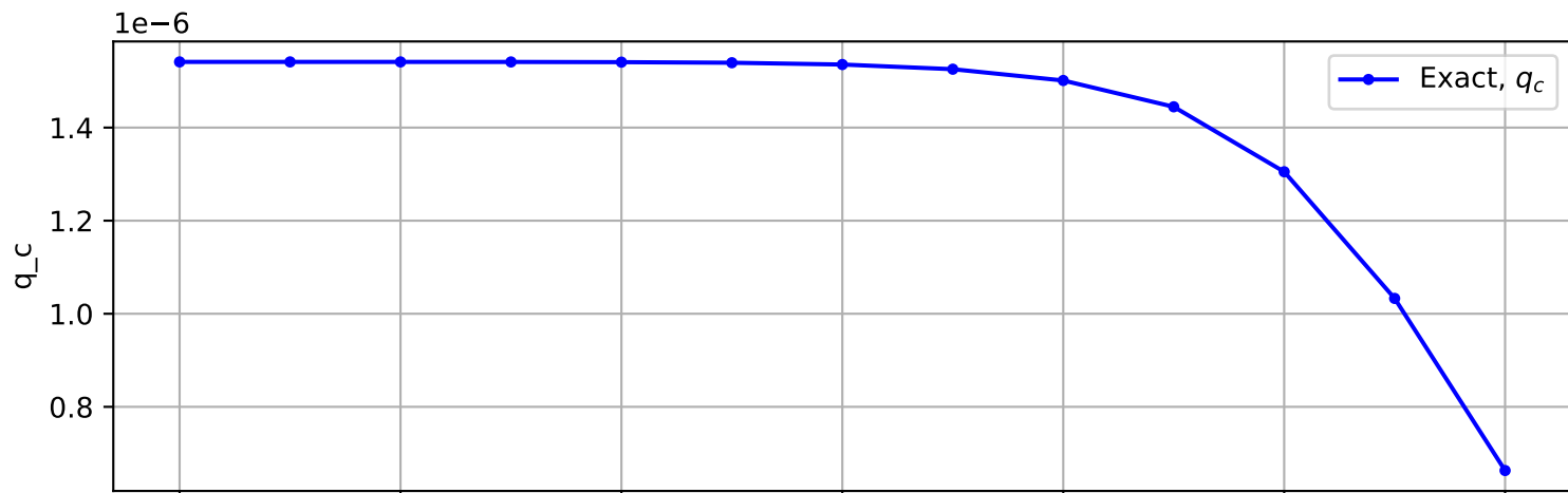
Trajectory No. 836
