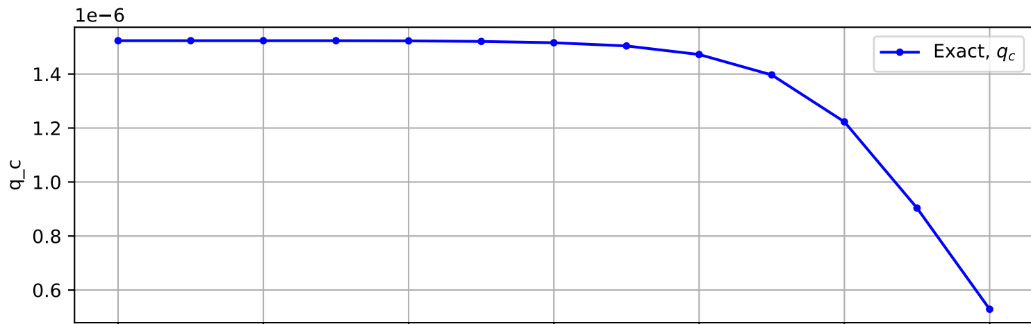
Trajectory No. 839
