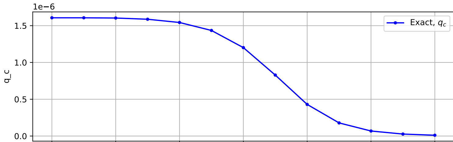
Trajectory No. 848
