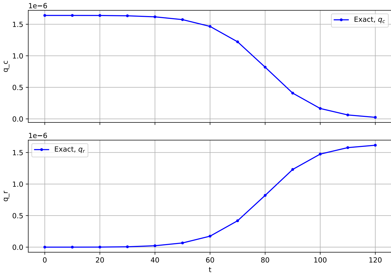
Trajectory No. 864
