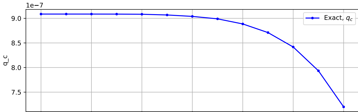
Trajectory No. 89
