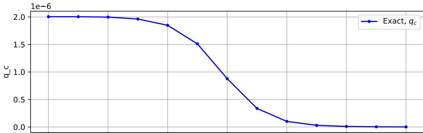
Trajectory No. 892
