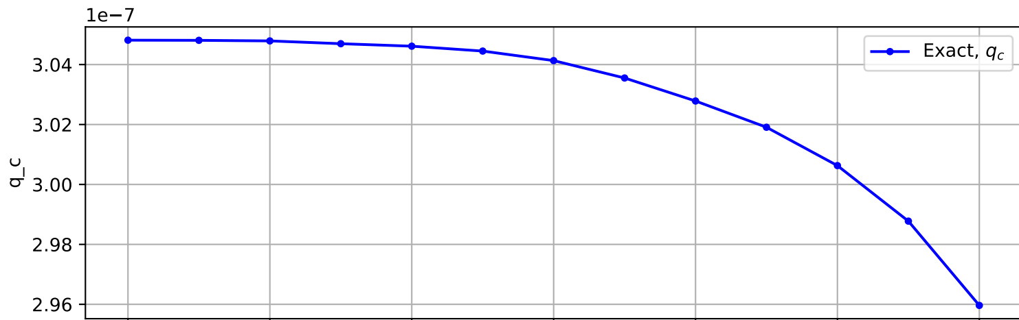
Trajectory No. 925
