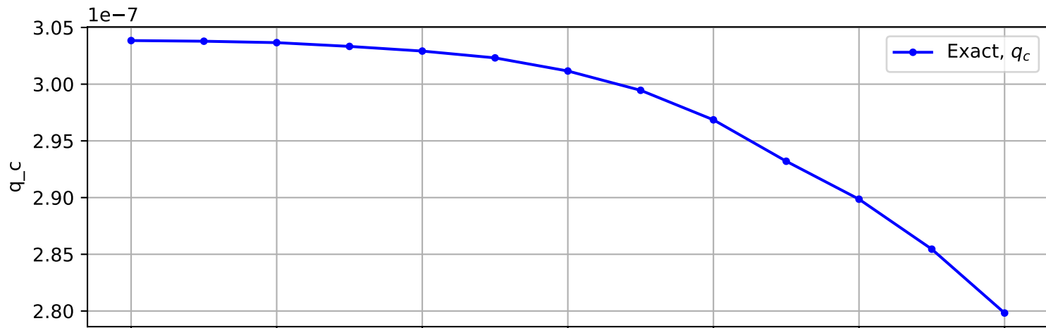
Trajectory No. 930
