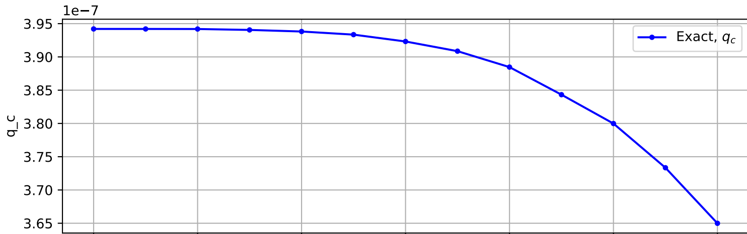
Trajectory No. 968
