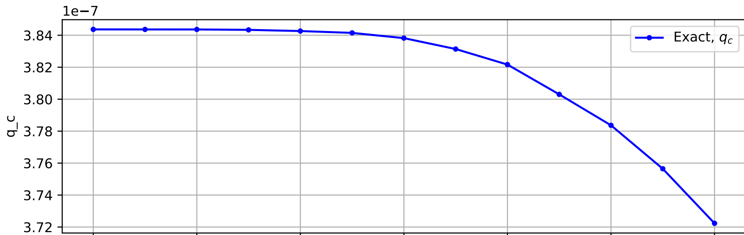
Trajectory No. 971
