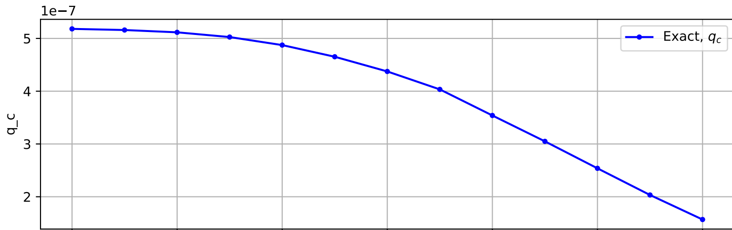
Trajectory No. 976
