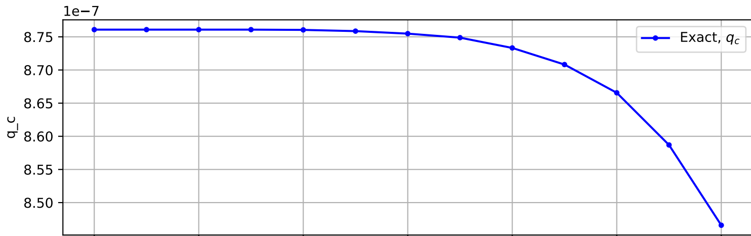
Trajectory No. 99
