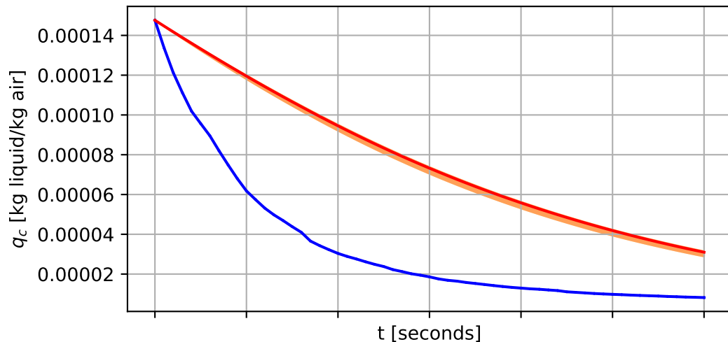
Trajectory No. 254
