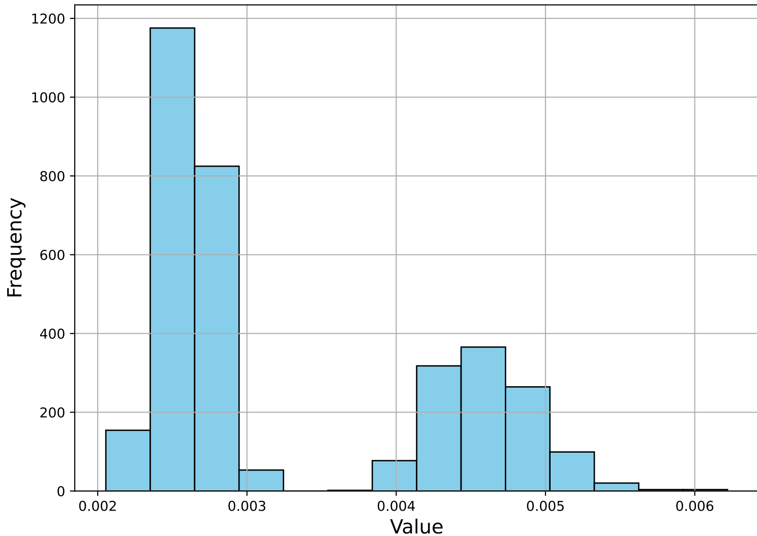
Variable 0, feature 3: x0 x1
