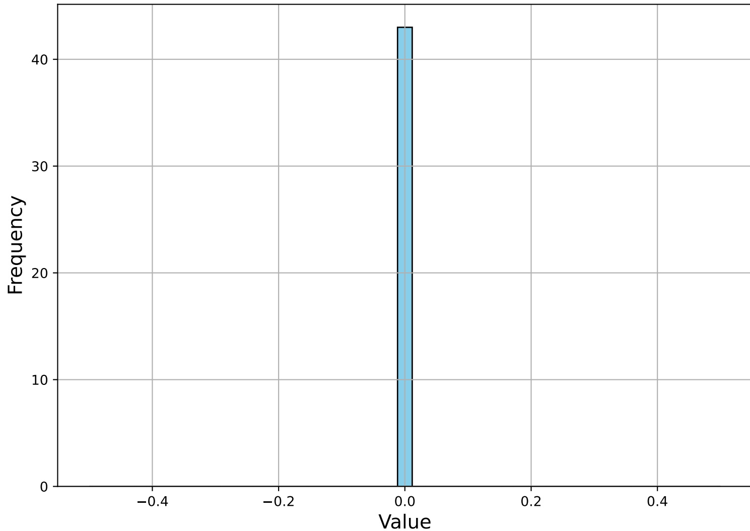
Variable 1, feature 5: x_0^3
