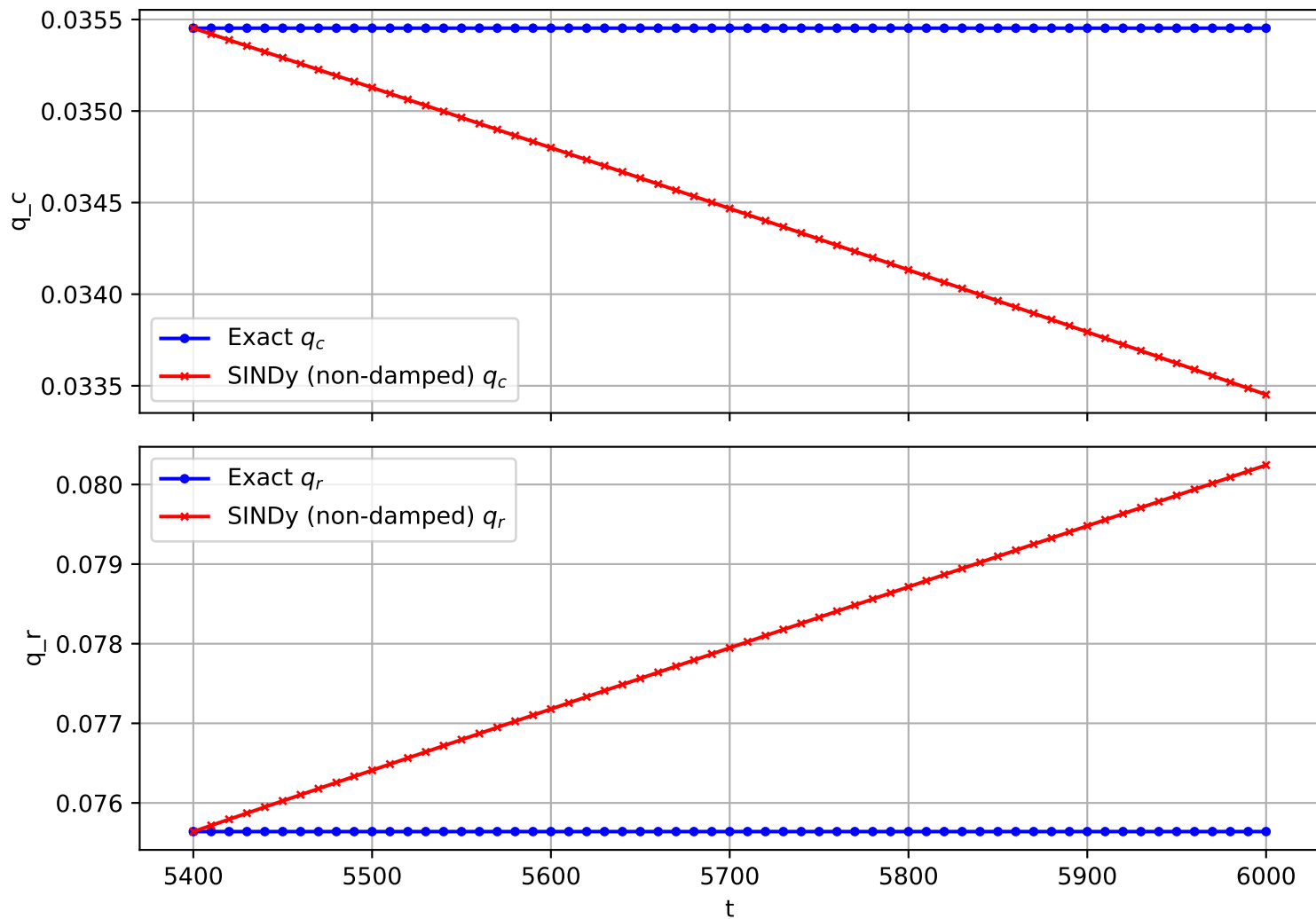
Trajectory 1 (non-damped)
