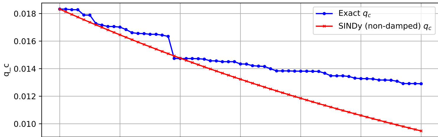
Trajectory 126 (non-damped)
