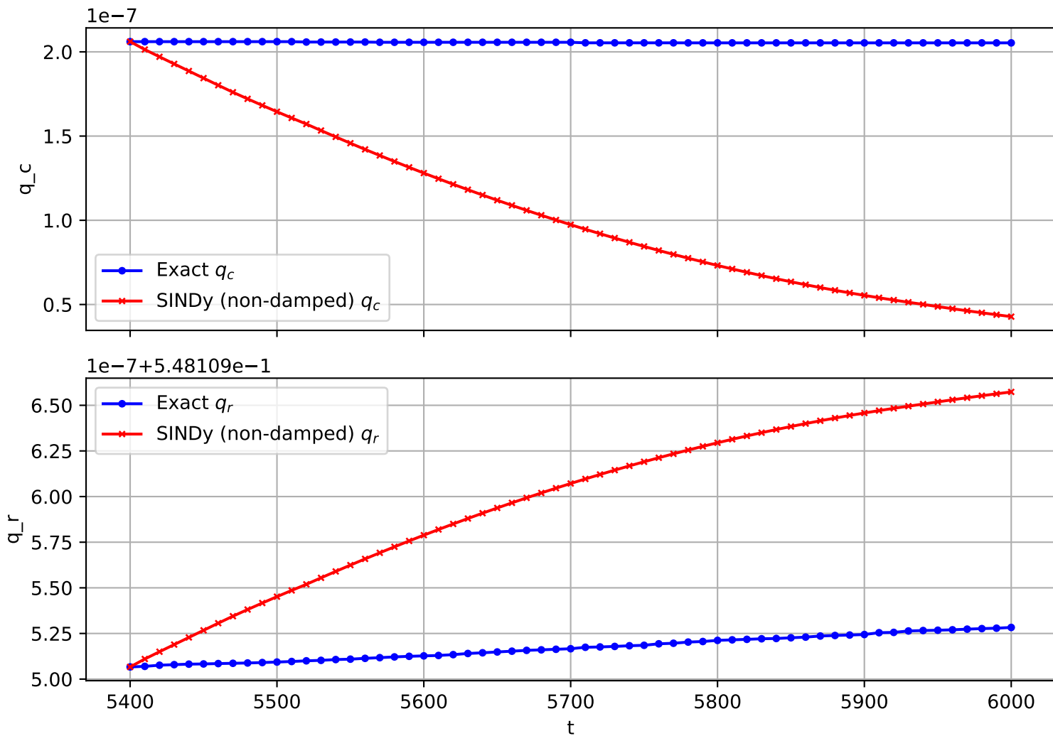
Trajectory 131 (non-damped)
