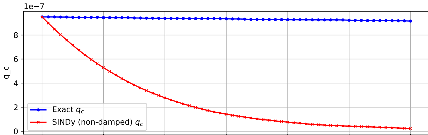
Trajectory 132 (non-damped)
