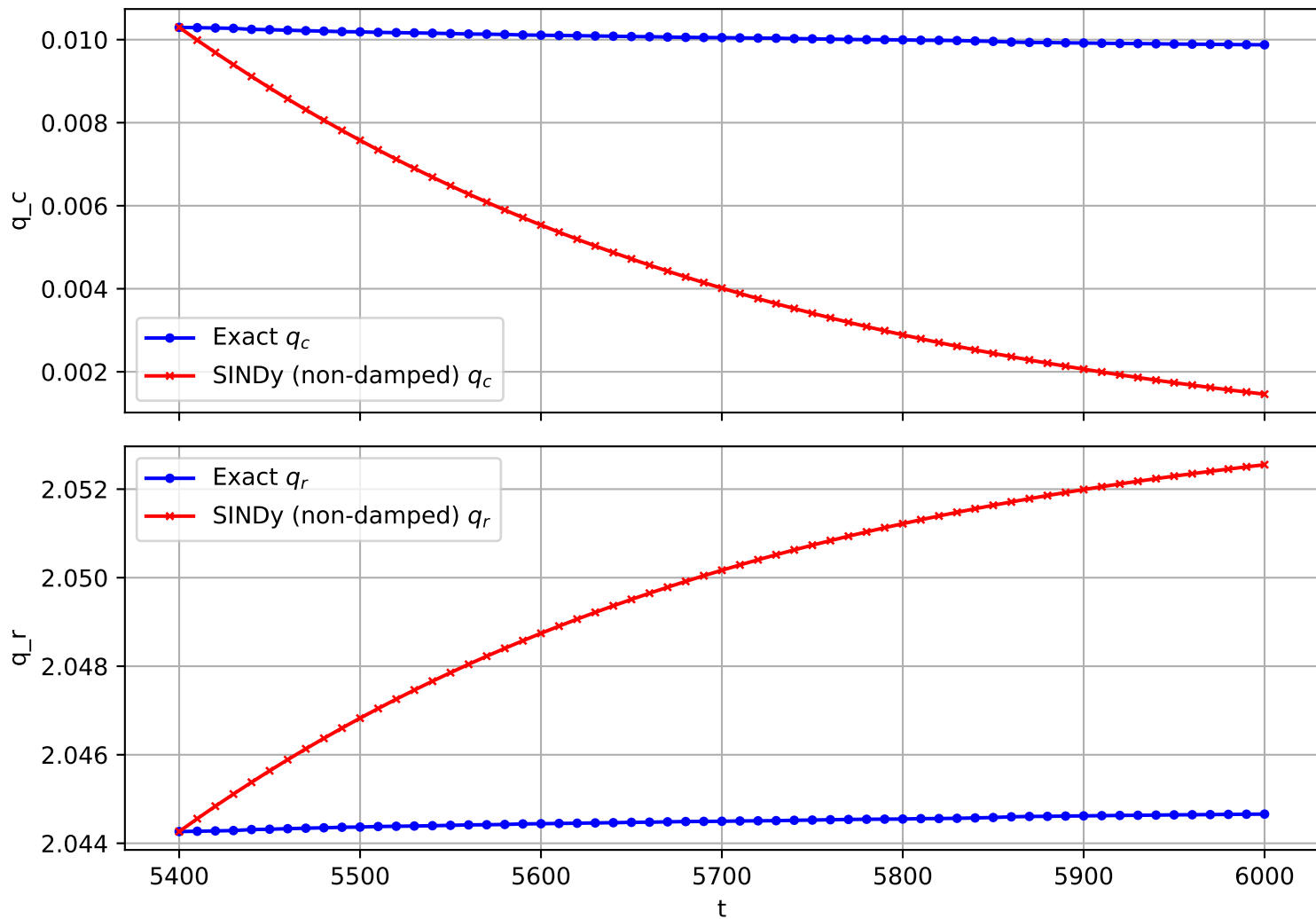
Trajectory 145 (non-damped)
