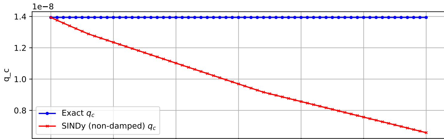
Trajectory 154 (non-damped)
