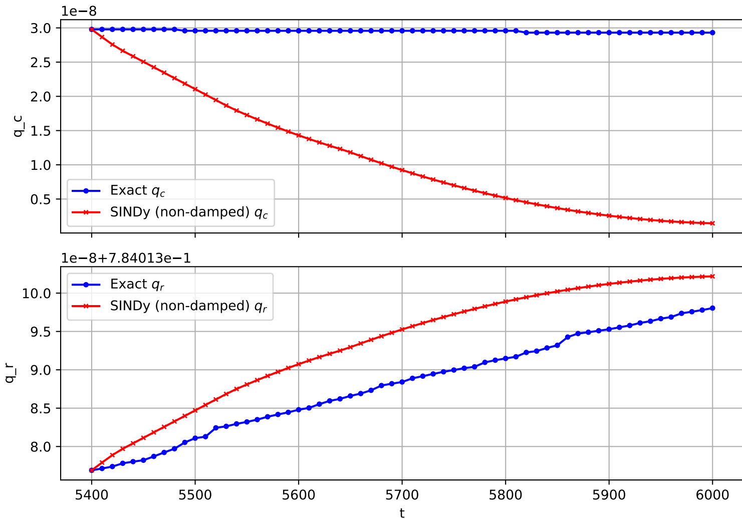
Trajectory 155 (non-damped)
