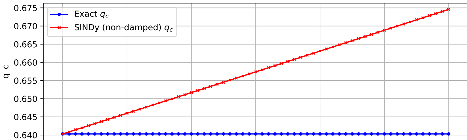
Trajectory 163 (non-damped)
