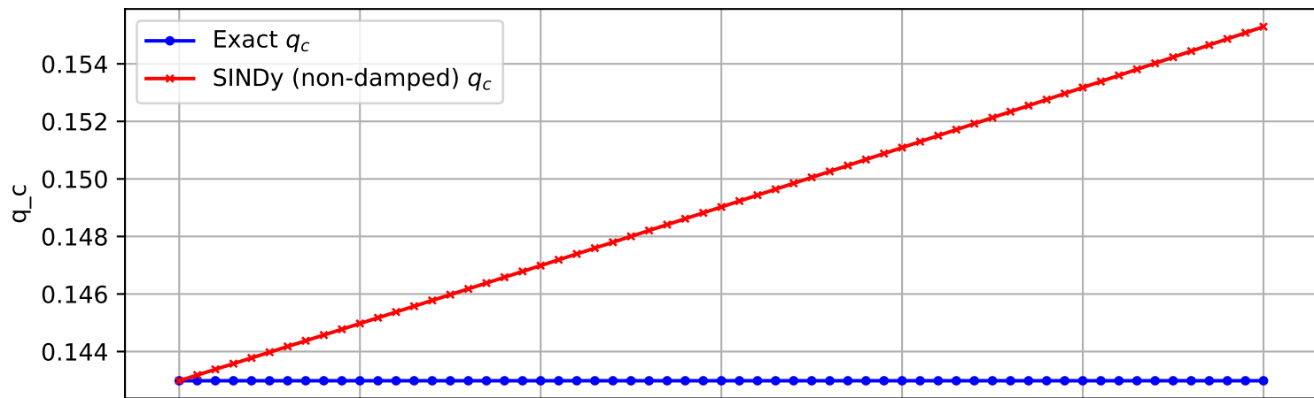
Trajectory 164 (non-damped)
