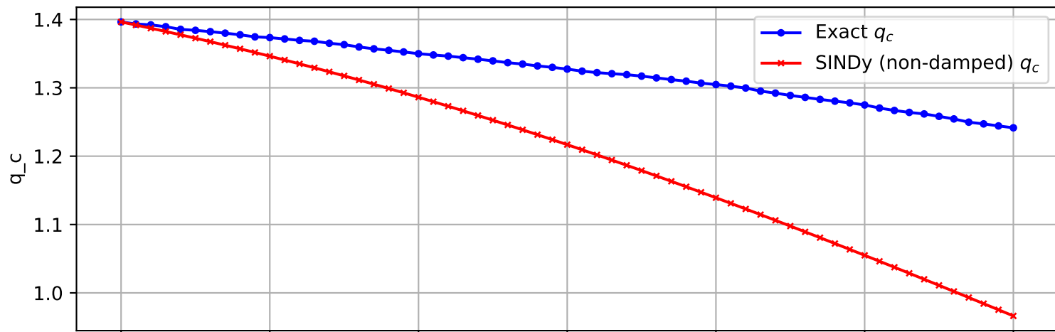
Trajectory 175 (non-damped)
